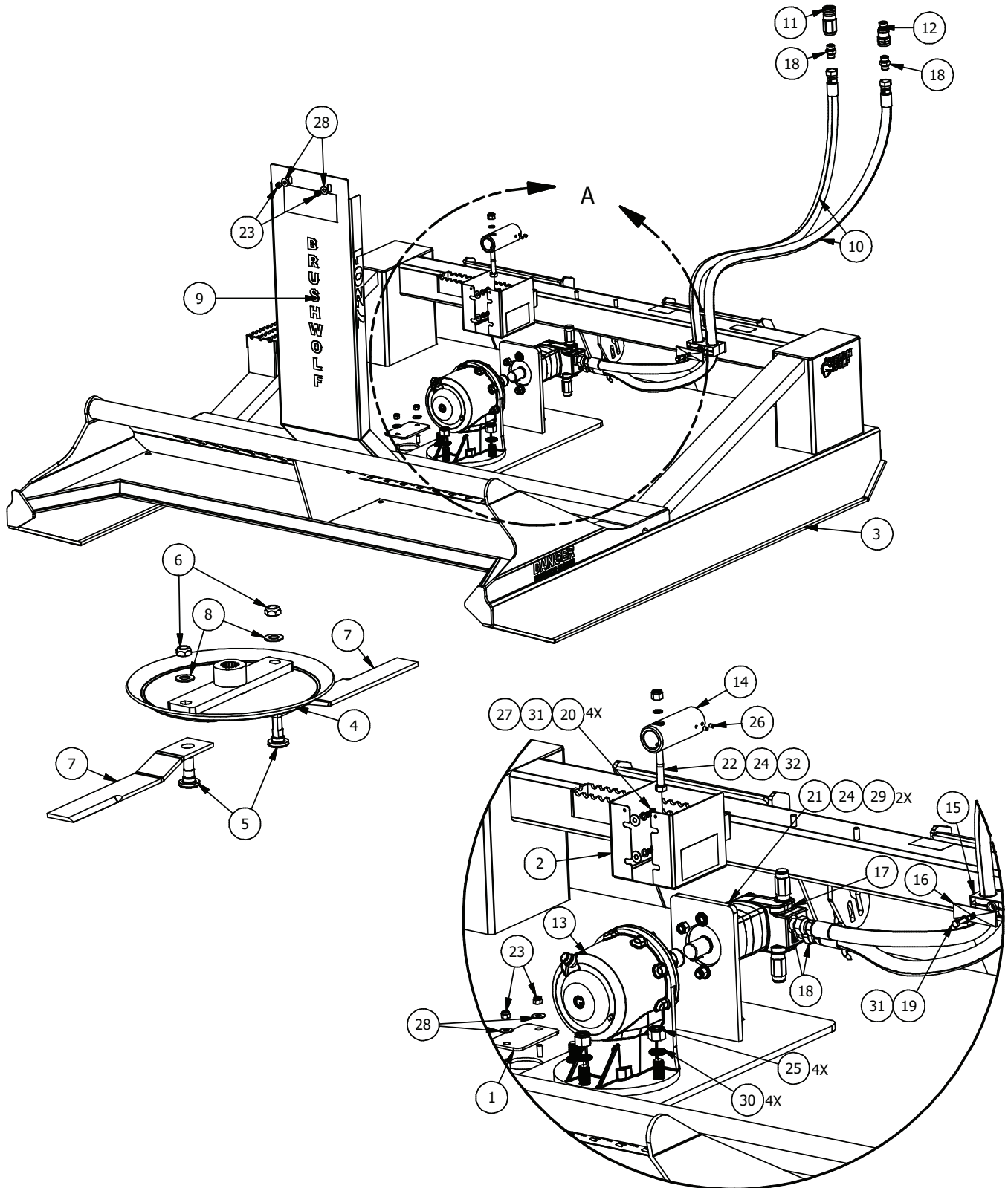
DETAIL A
